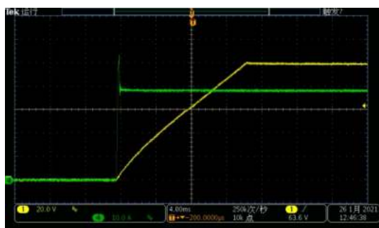
CV Priority (High-speed build-up voltage, current overshoot)
