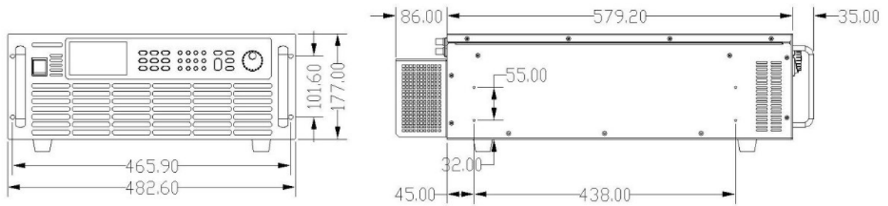
4U model (4kW、6kW) Dimension Drawing
