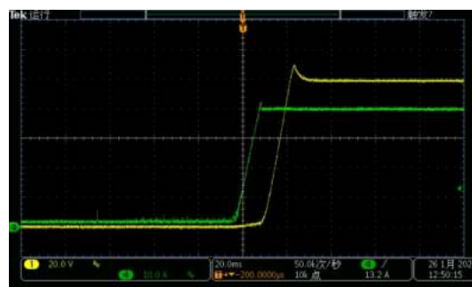
CC priority (High-speed build-up current, voltage overshoot)
