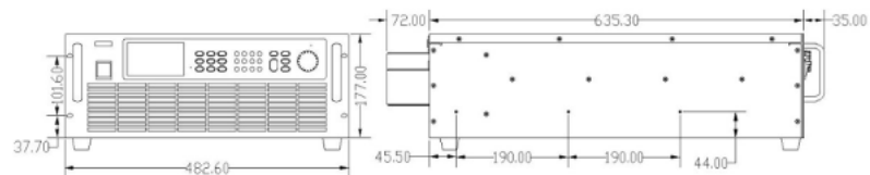
Dimension drawing of 30kW model
